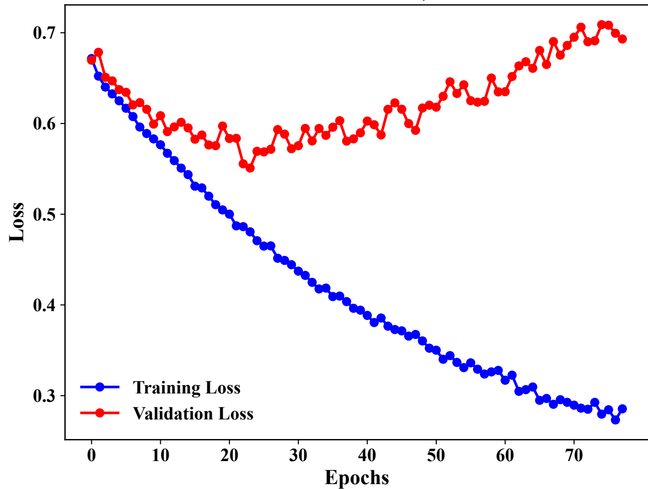
Loss Curves: Seed 64, Rank 1
